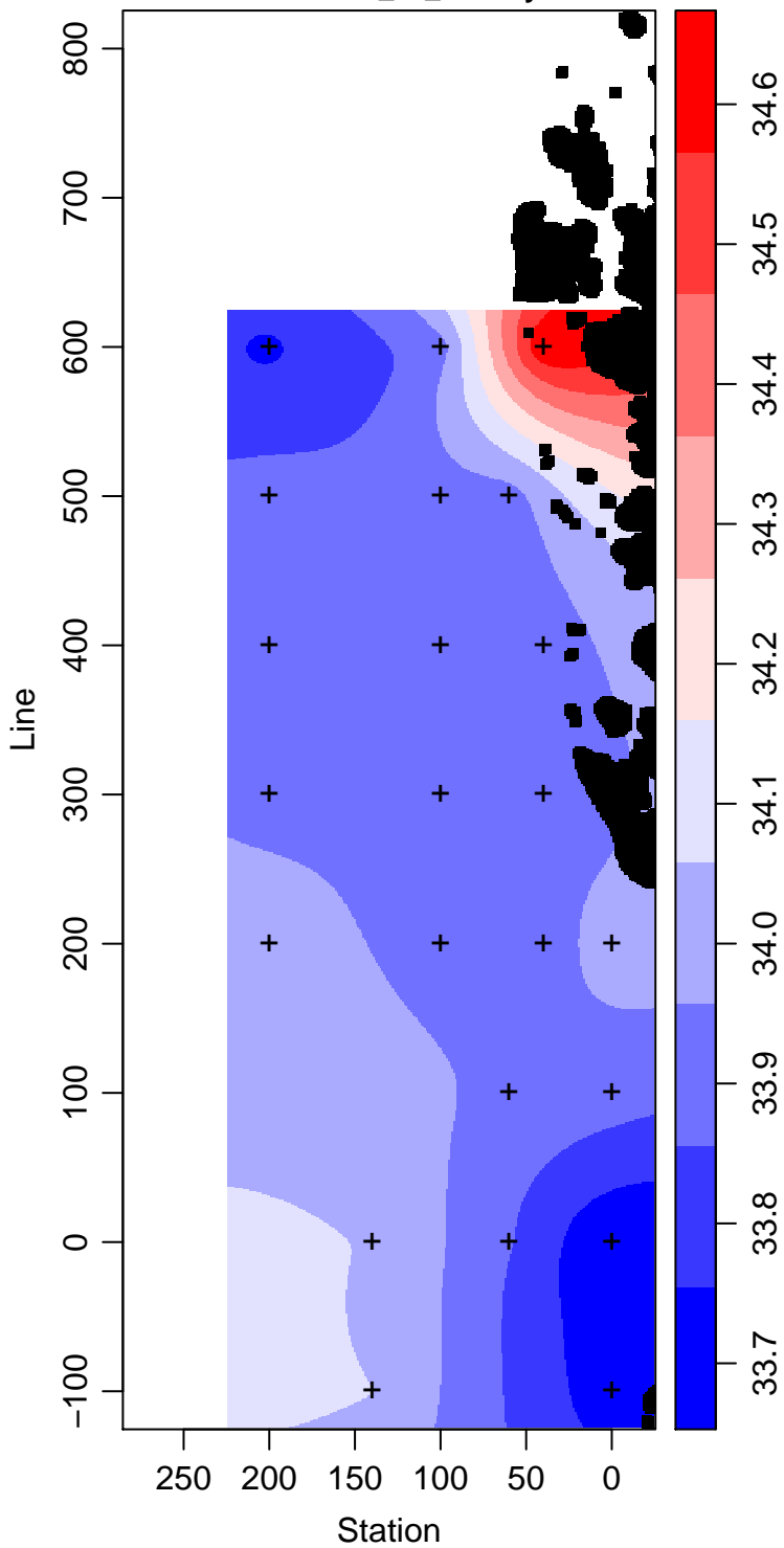
LMG13-01_50_Salinity
