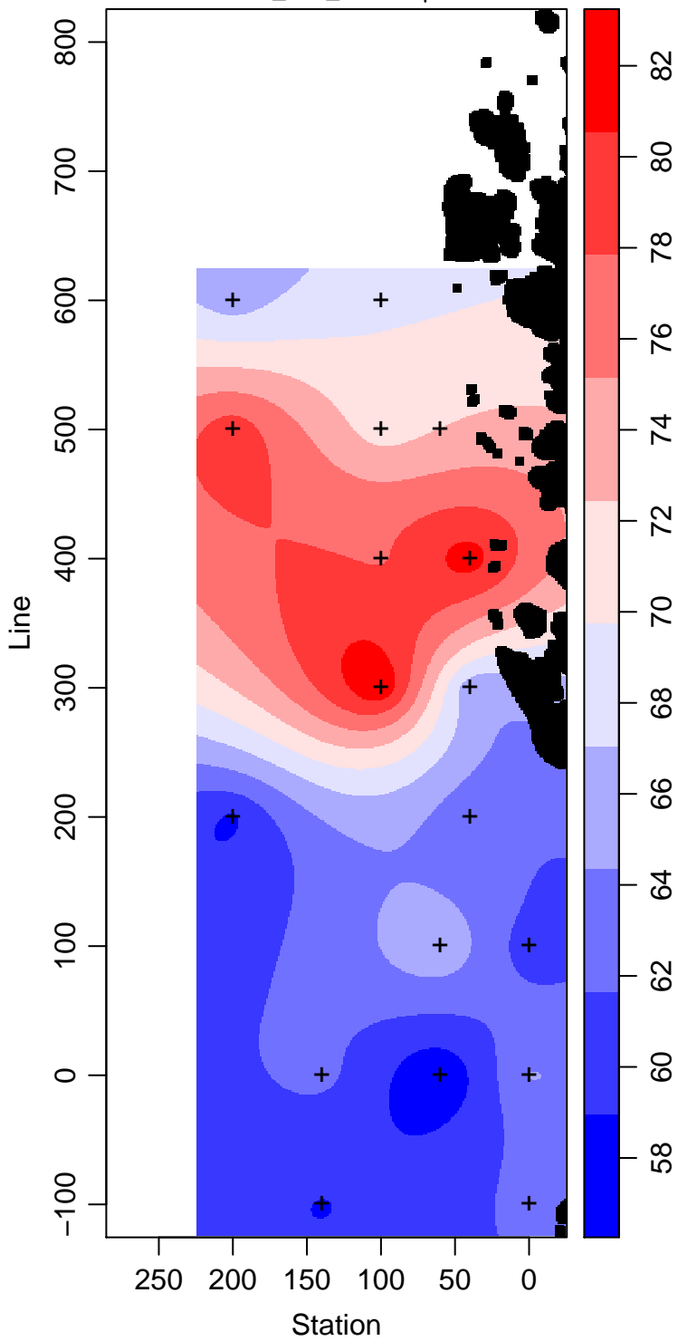
LMG13-01_100_Silicate \mu\text{ mol L}^{-1}
