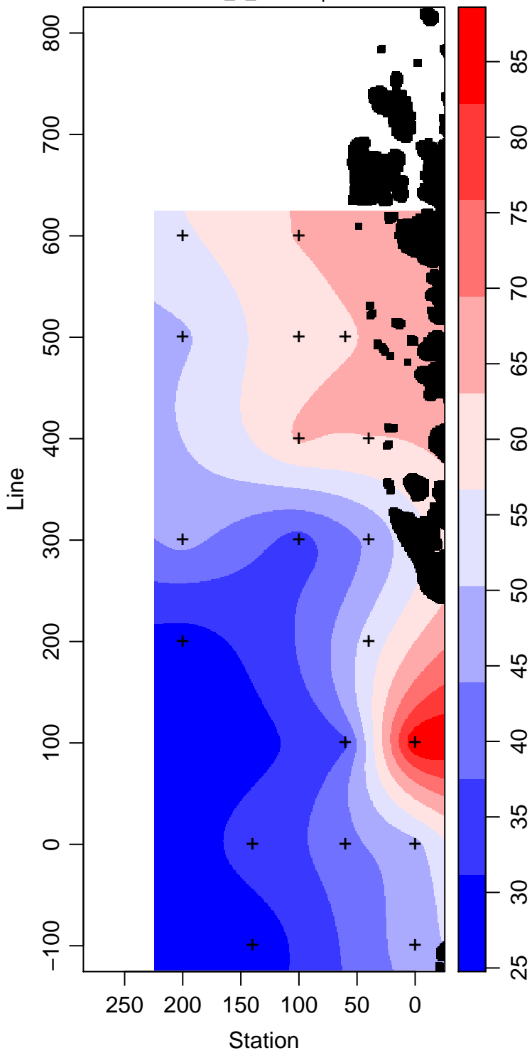
LMG13-01_1_Silicate \mu\text{ mol L}^{-1}
