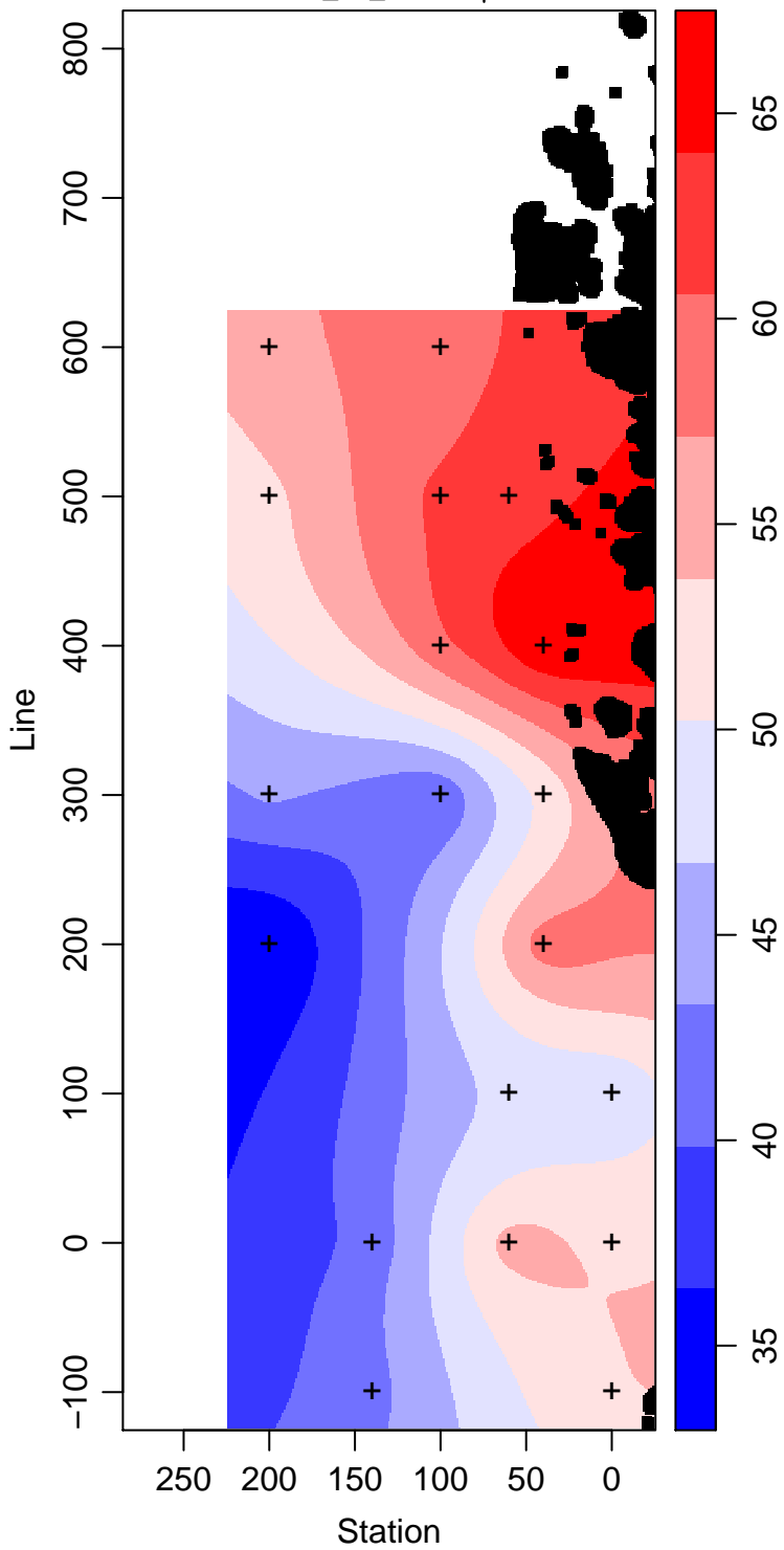
LMG13-01_25_Silicate \mu\text{ mol L}^{-1}
