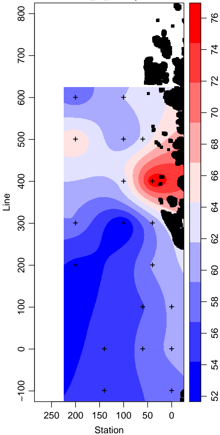
LMG13-01_60_Silicate \mu\text{ mol L}^{-1}
