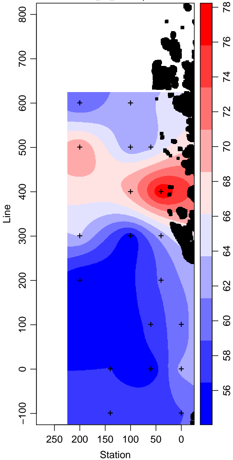
LMG13-01_70_Silicate \mu\text{ mol L}^{-1}
