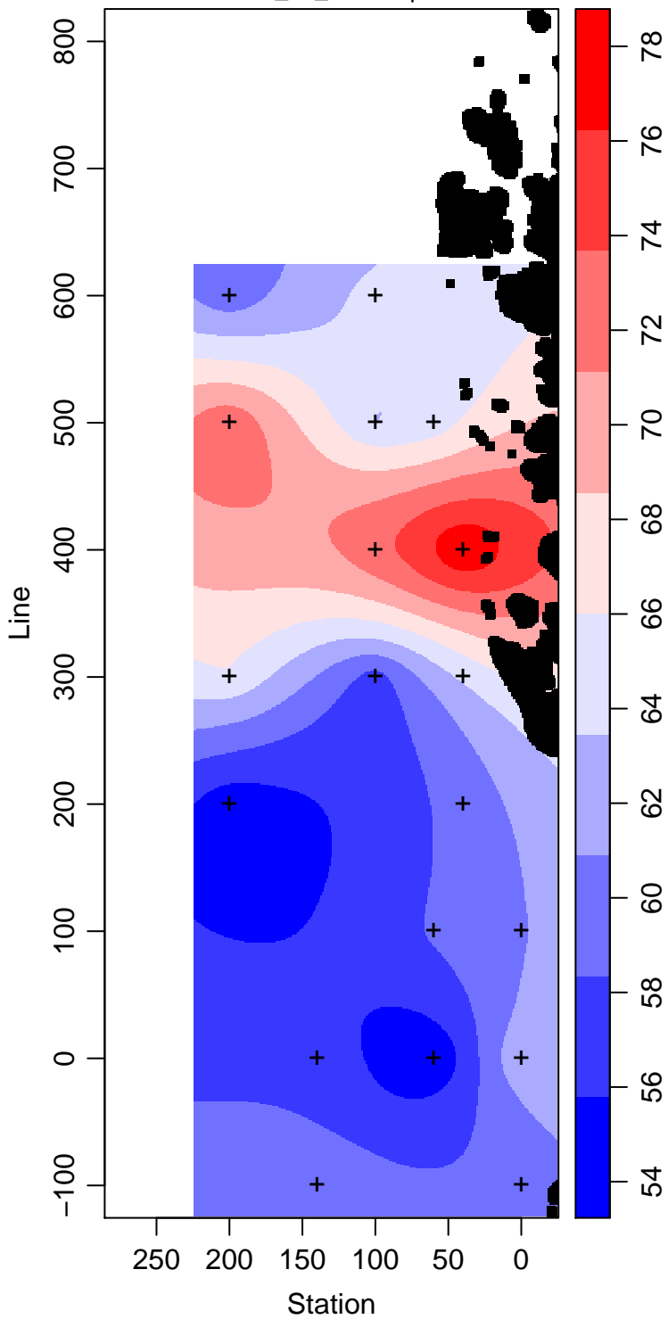
LMG13-01_75_Silicate \mu\text{ mol L}^{-1}
