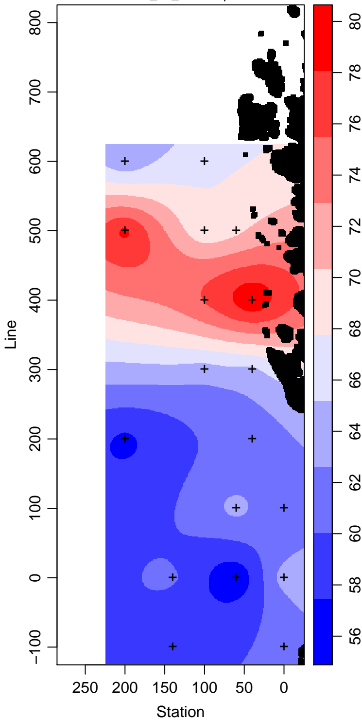
LMG13-01_90_Silicate \mu\text{ mol L}^{-1}
