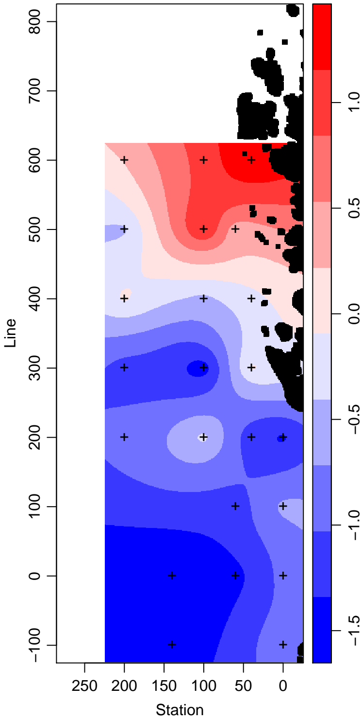
LMG13-01_25_Temperature ° Celsius
