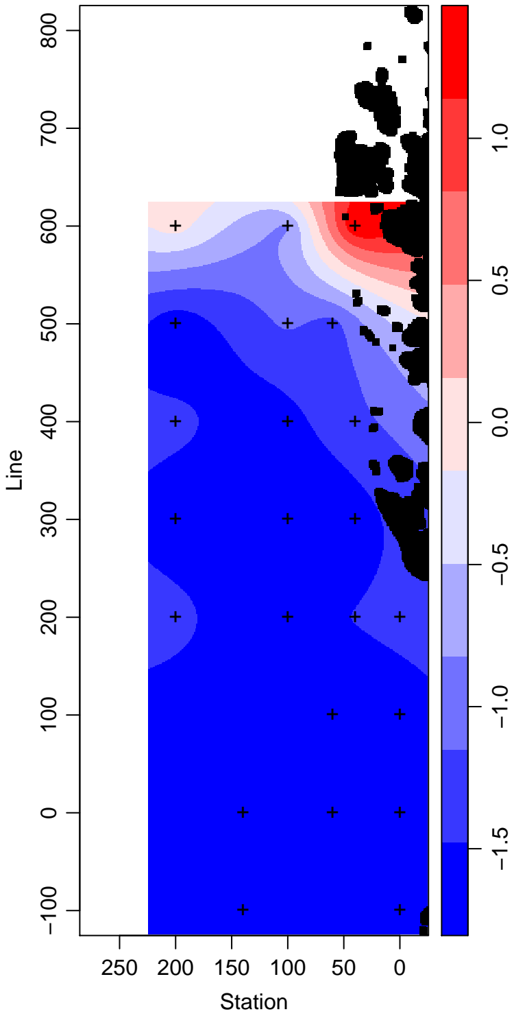
LMG13-01_55_Temperature ° Celsius
