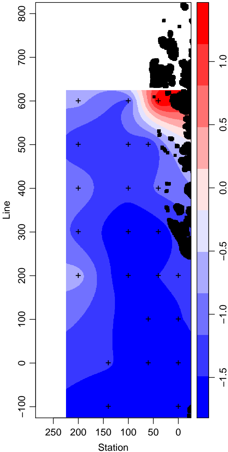
LMG13-01_70_Temperature ° Celsius
