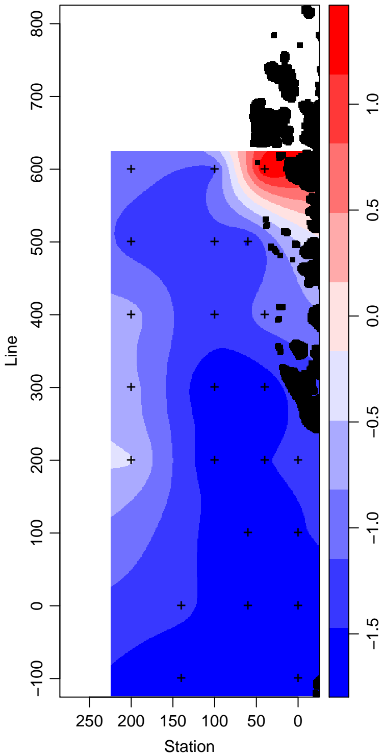
LMG13-01_75_Temperature ° Celsius
