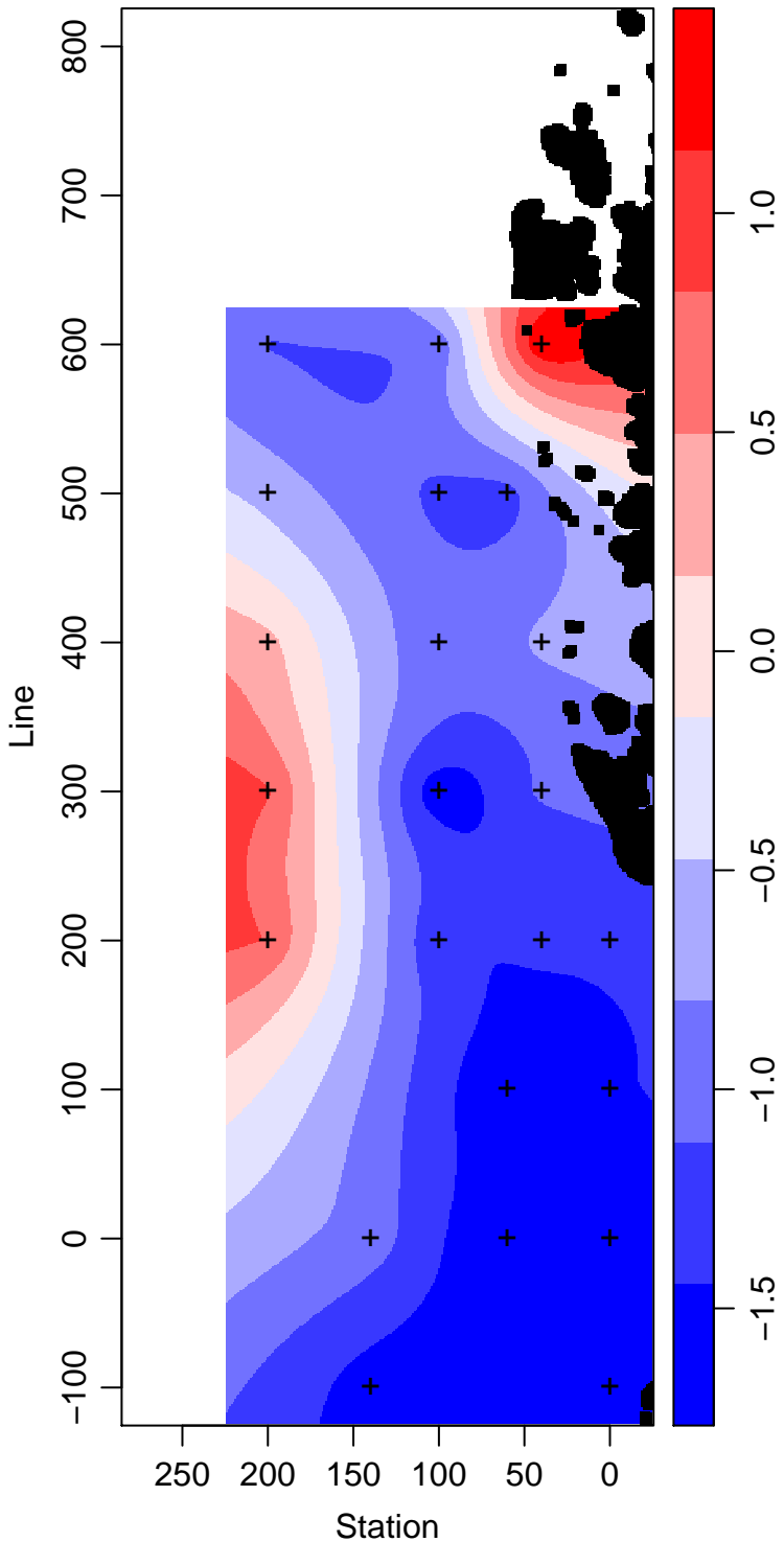
LMG13-01_95_Temperature ° Celsius
