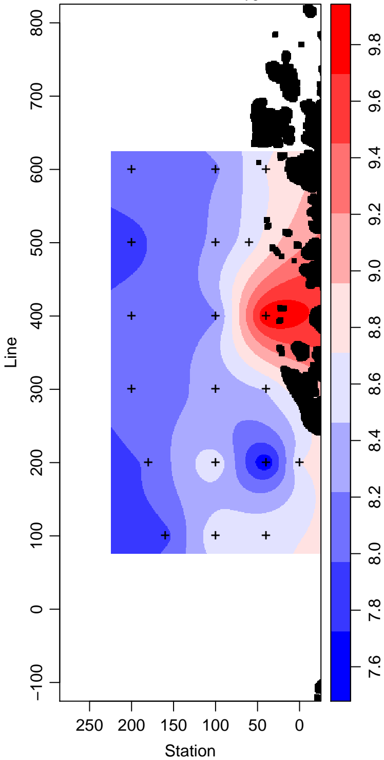
LMG14-01_15_Dissolved.Oxygen ml L -1
