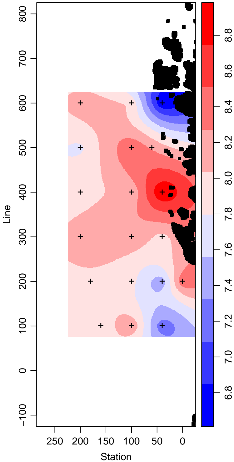
LMG14-01_20_Dissolved.Oxygen ml L -1
