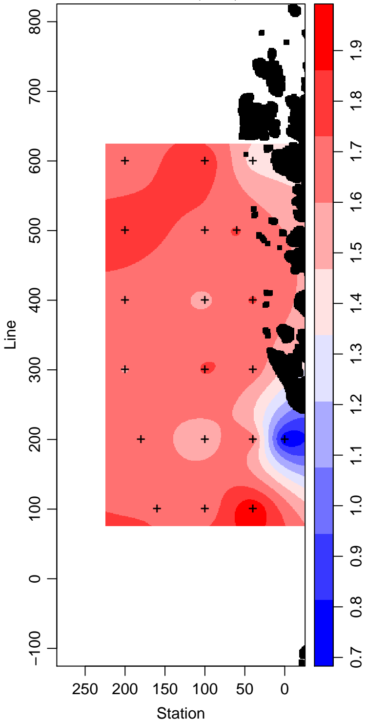
LMG14-01_20_Phosphate \mu\text{ mol L}^{-1}
