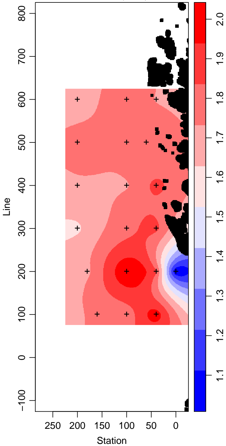
LMG14-01_25_Phosphate \mu\text{ mol L}^{-1}
