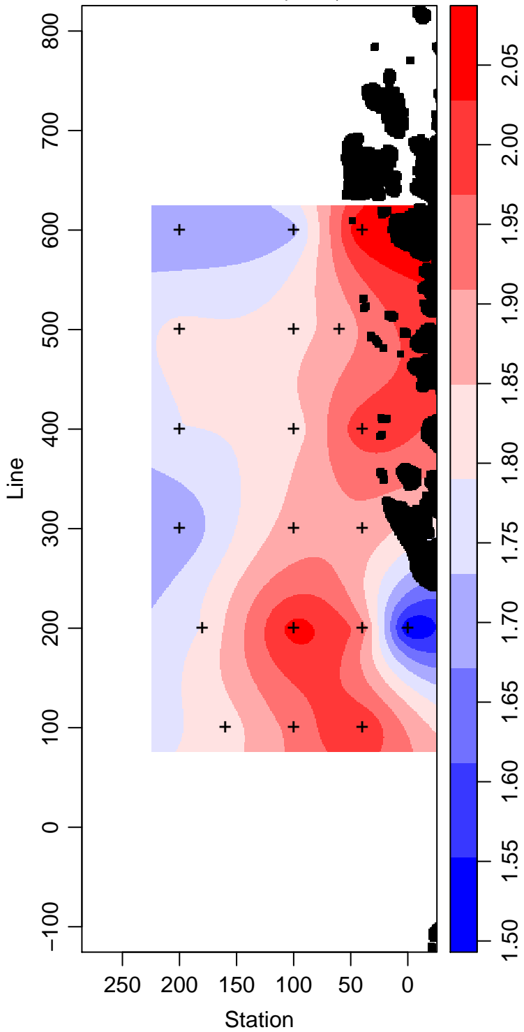
LMG14-01_35_Phosphate \mu\text{ mol L}^{-1}
