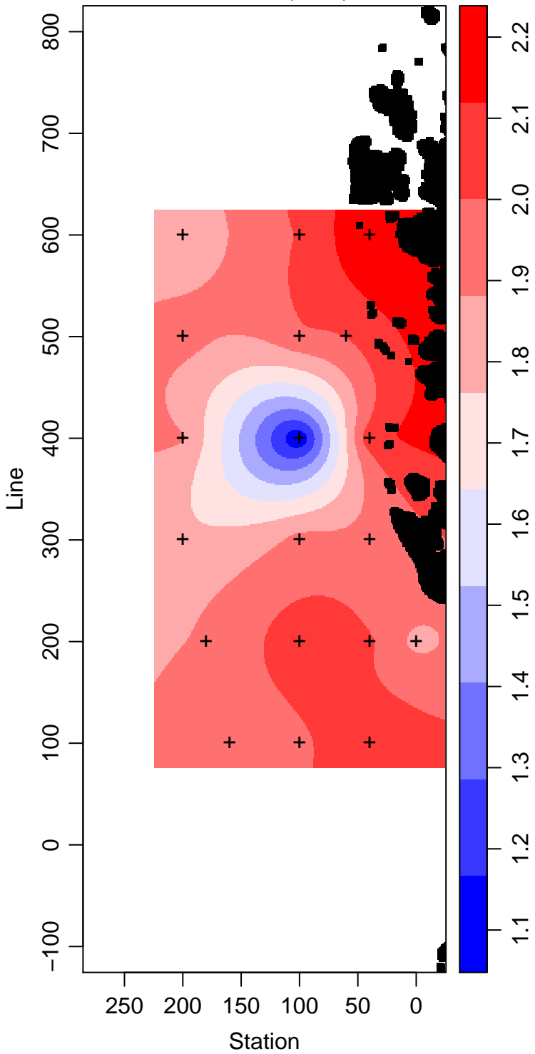
LMG14-01_50_Phosphate \mu\text{ mol L}^{-1}
