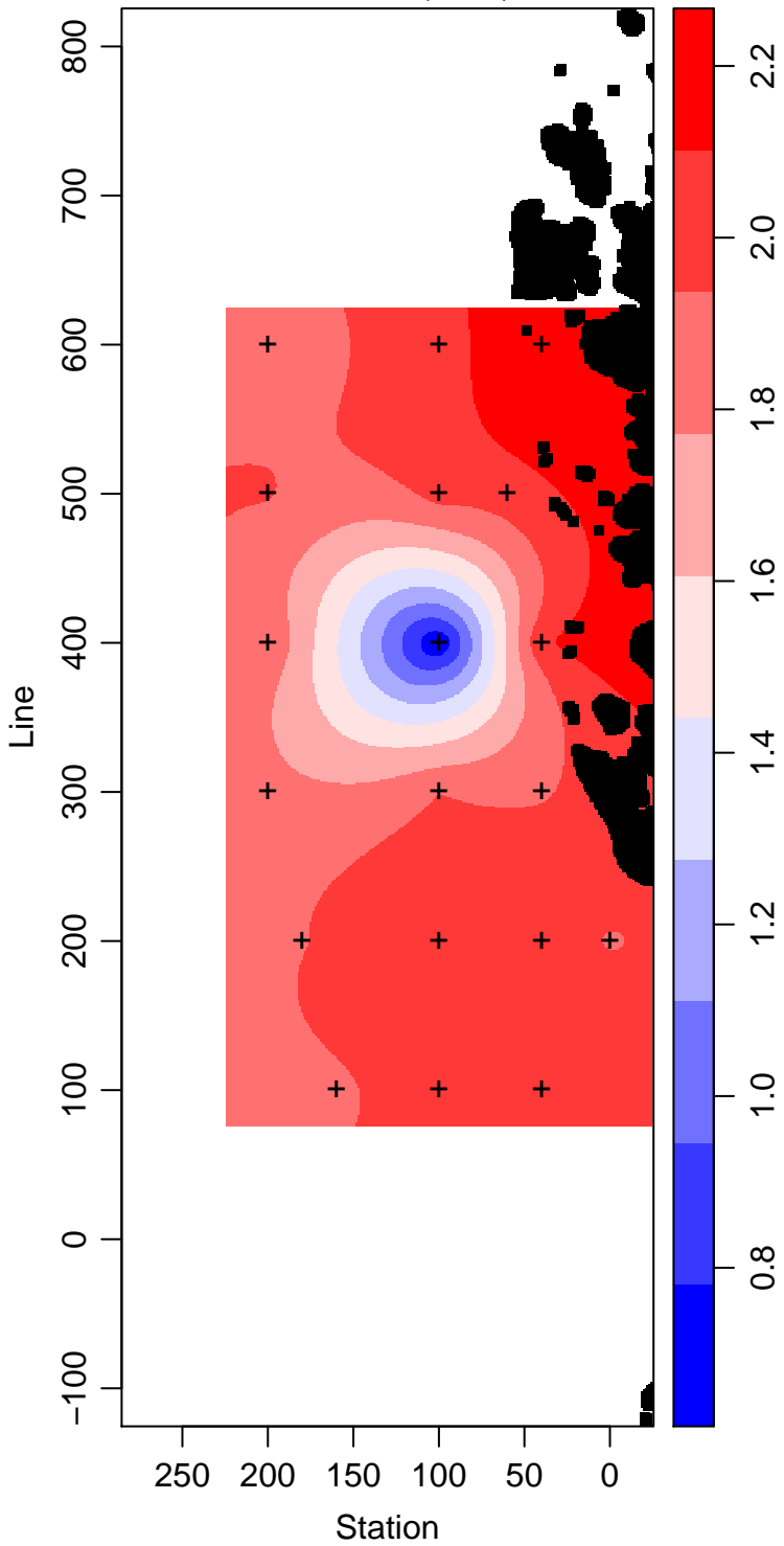
LMG14-01_55_Phosphate \mu\text{ mol L}^{-1}
