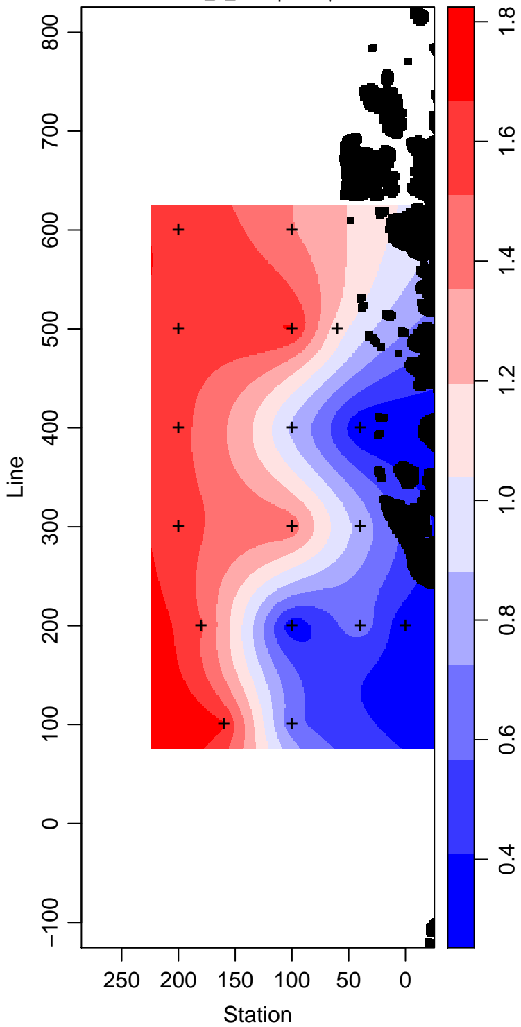
LMG14-01_5_Phosphate \mu\text{ mol L}^{-1}
