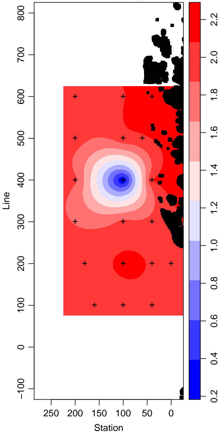
LMG14-01_60_Phosphate \mu\text{ mol L}^{-1}
