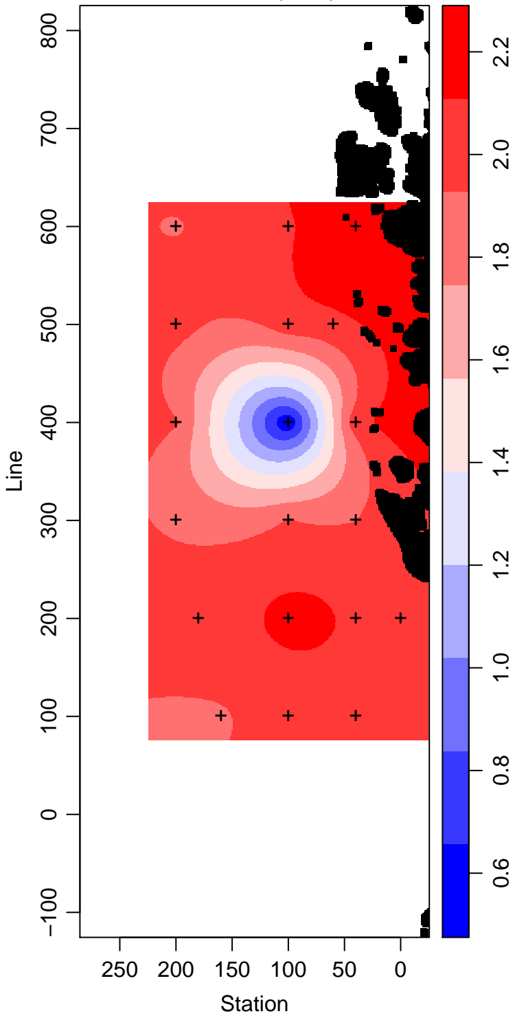
LMG14-01_65_Phosphate \mu\text{ mol L}^{-1}
