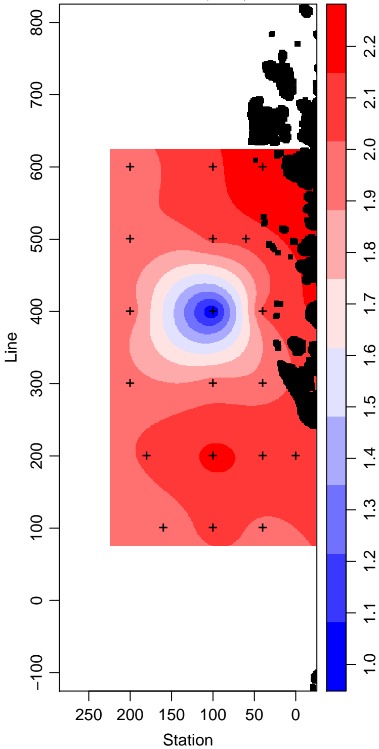
LMG14-01_70_Phosphate \mu\text{ mol L}^{-1}
