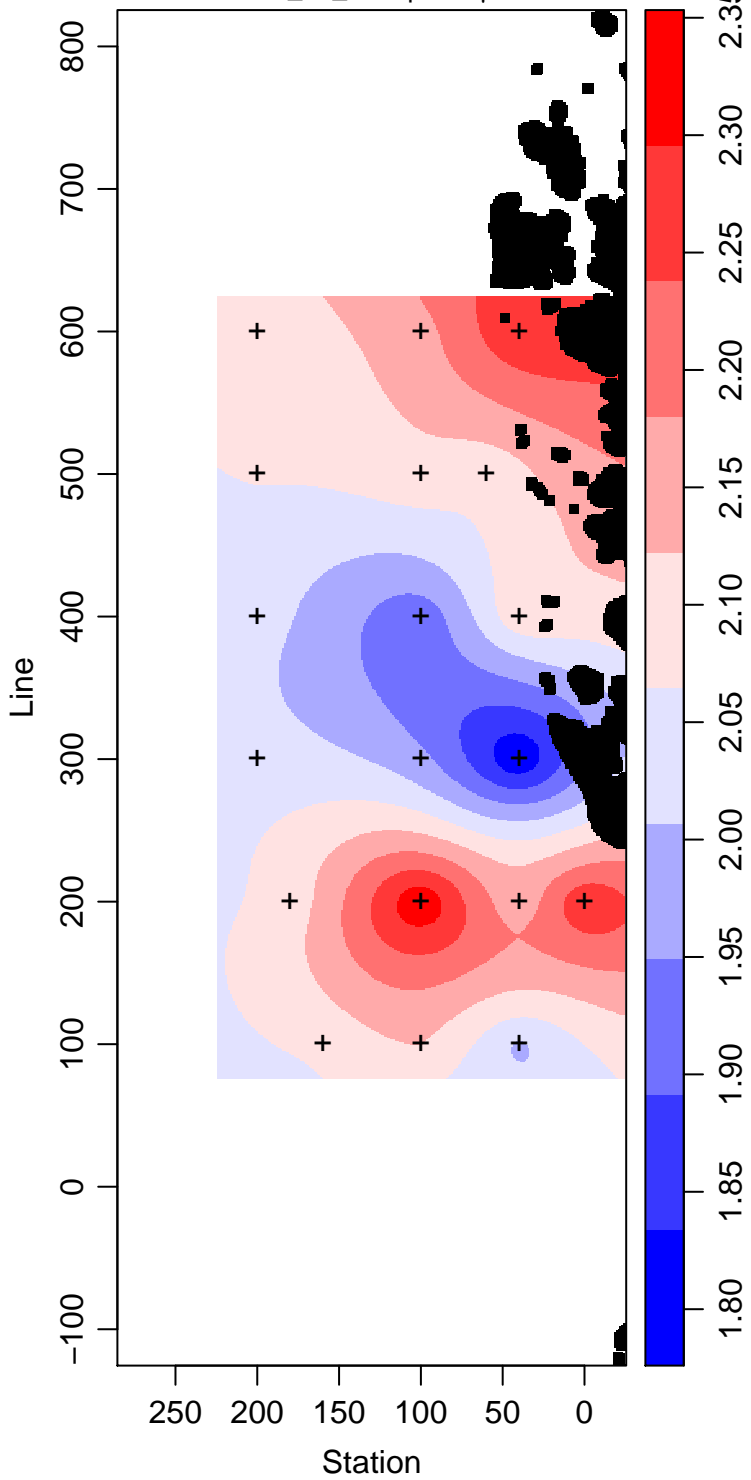
LMG14-01_90_Phosphate \mu\text{ mol L}^{-1}
