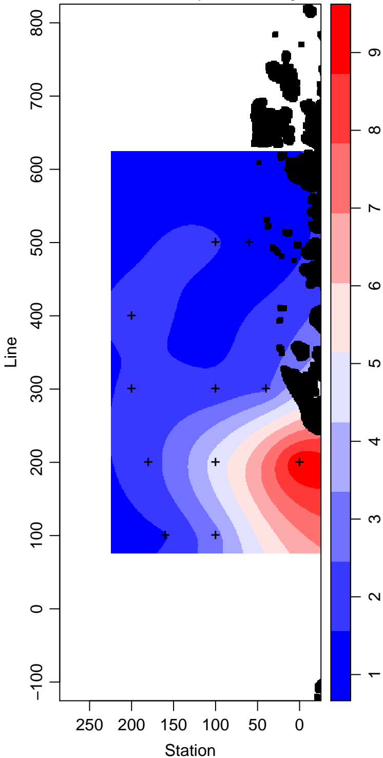
LMG14-01_70_Primary.Production mg m -3
