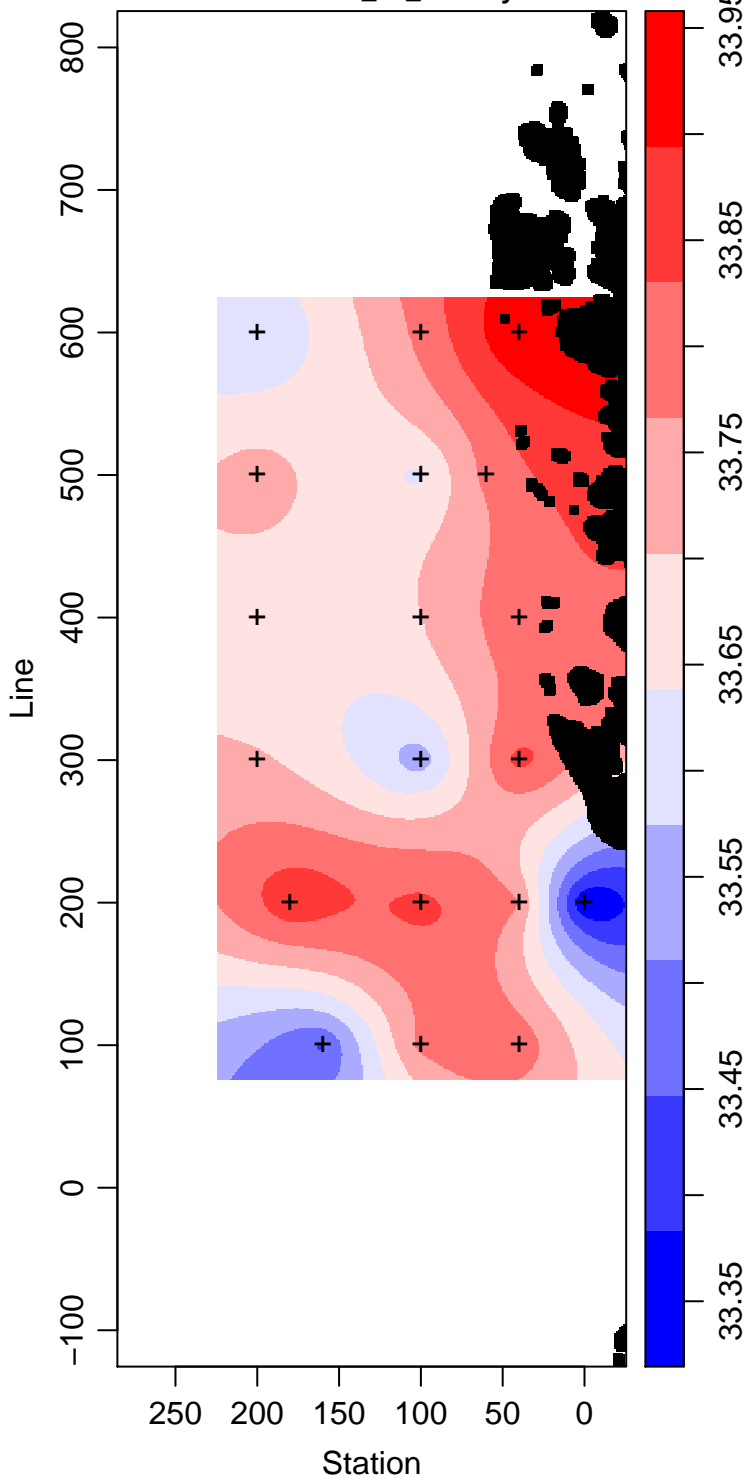
LMG14-01_30_Salinity
