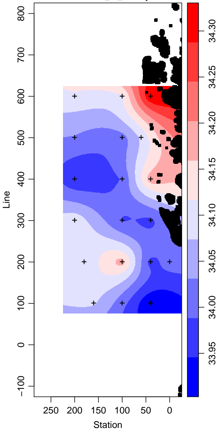
LMG14-01_90_Salinity
