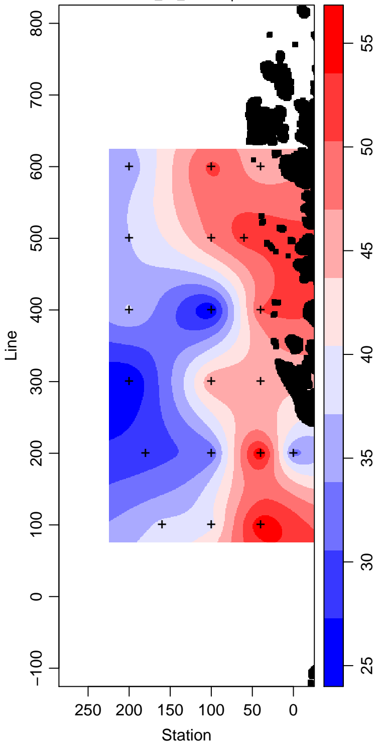
LMG14-01_10_Silicate \mu\text{ mol L}^{-1}
