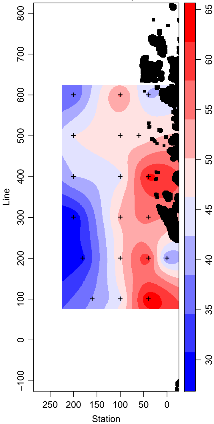
LMG14-01_20_Silicate \mu\text{ mol L}^{-1}
