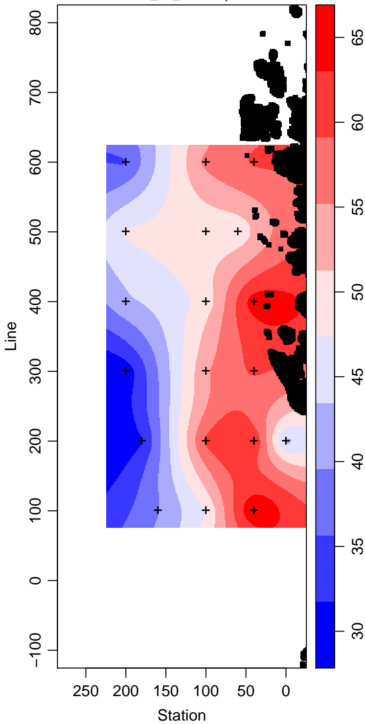
LMG14-01_25_Silicate \mu\text{ mol L}^{-1}
