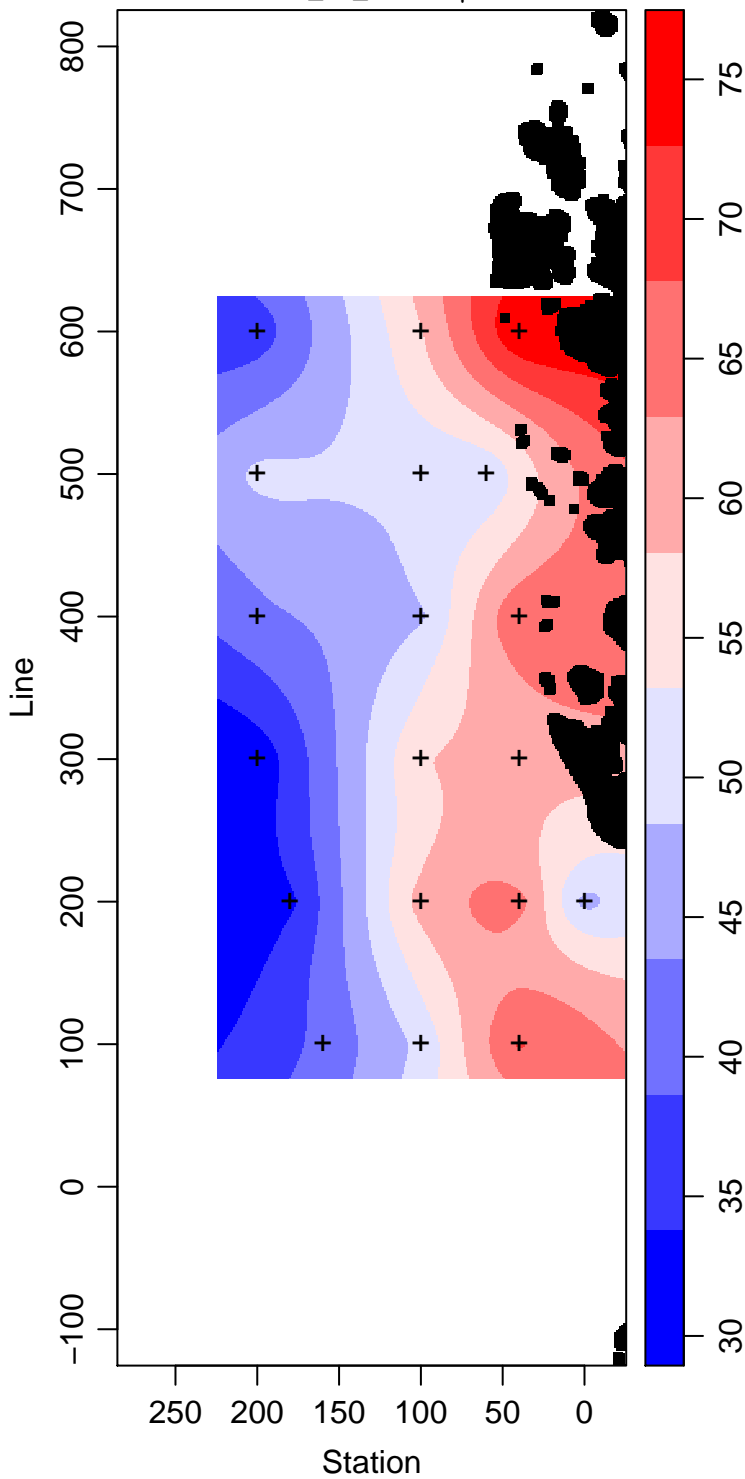
LMG14-01_30_Silicate \mu\text{ mol L}^{-1}
