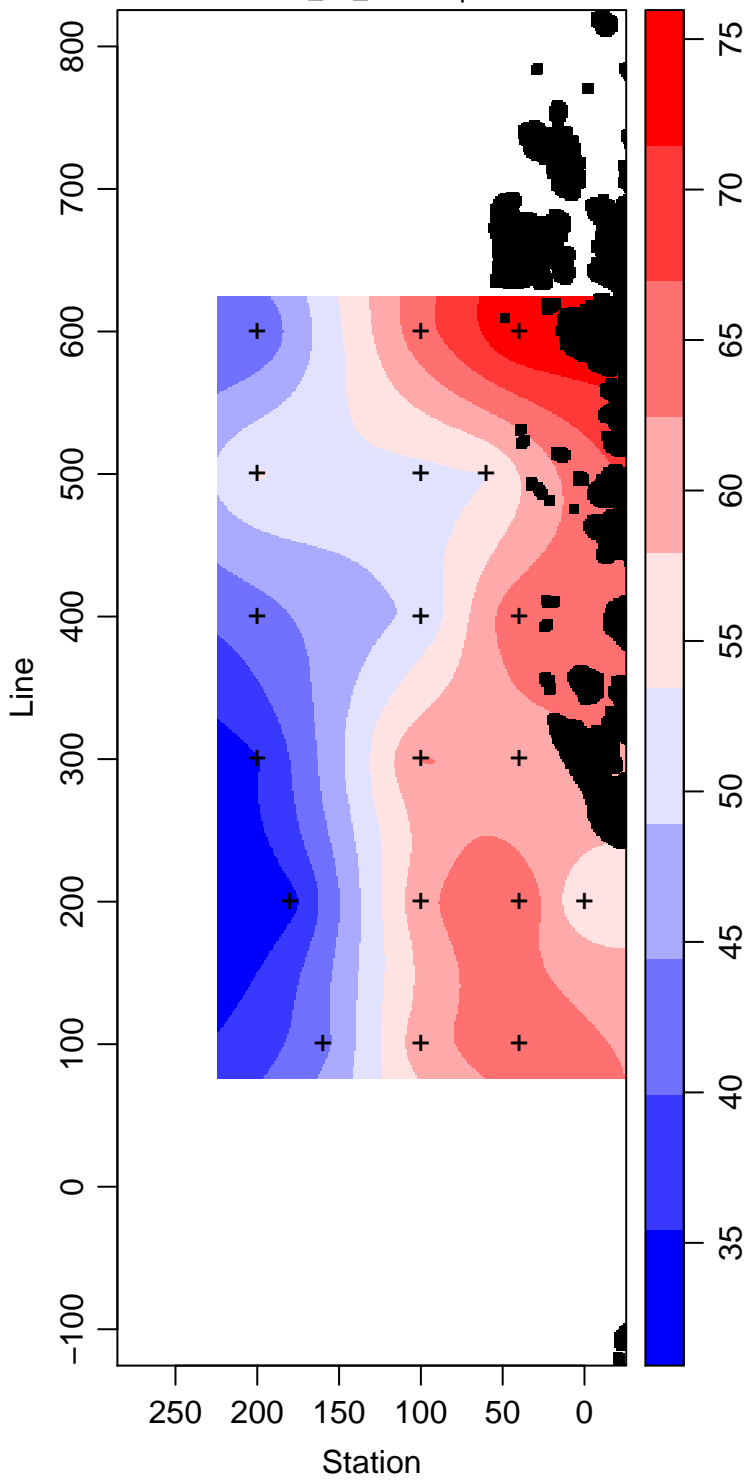
LMG14-01_55_Silicate \mu\text{ mol L}^{-1}
