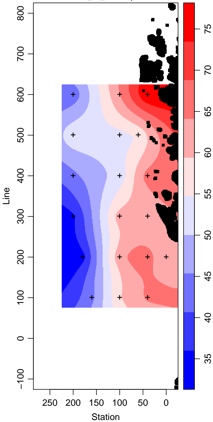
LMG14-01_65_Silicate \mu\text{ mol L}^{-1}
