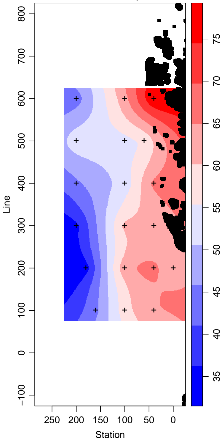
LMG14-01_70_Silicate \mu\text{ mol L}^{-1}
