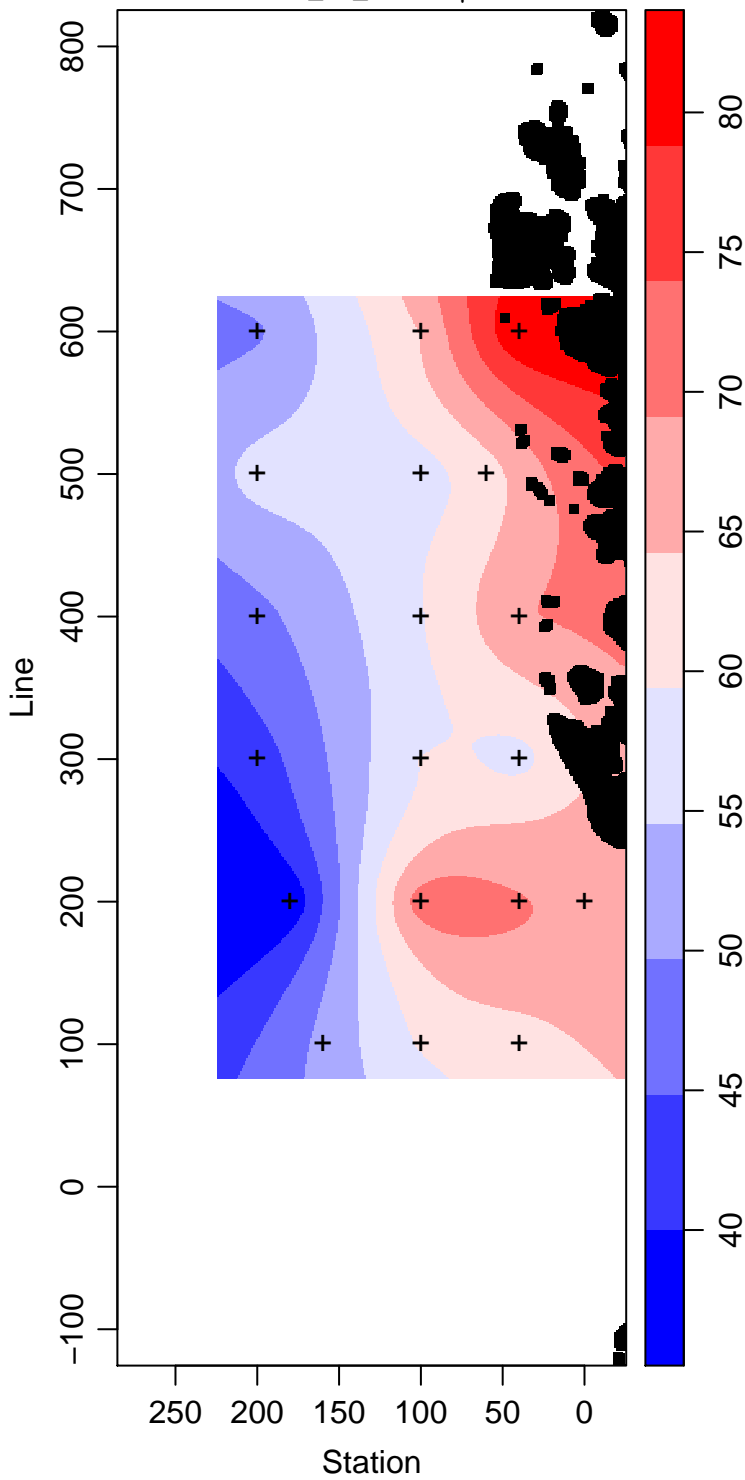
LMG14-01_90_Silicate \mu\text{ mol L}^{-1}
