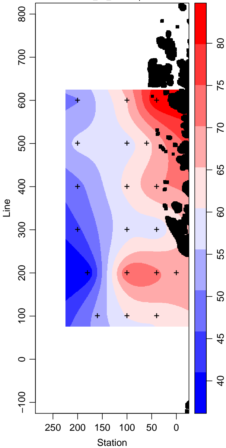
LMG14-01_95_Silicate \mu\text{ mol L}^{-1}
