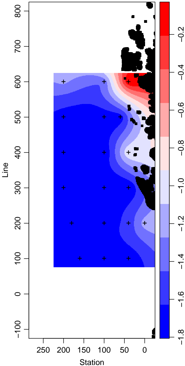
LMG14-01_60_Temperature ° Celsius
