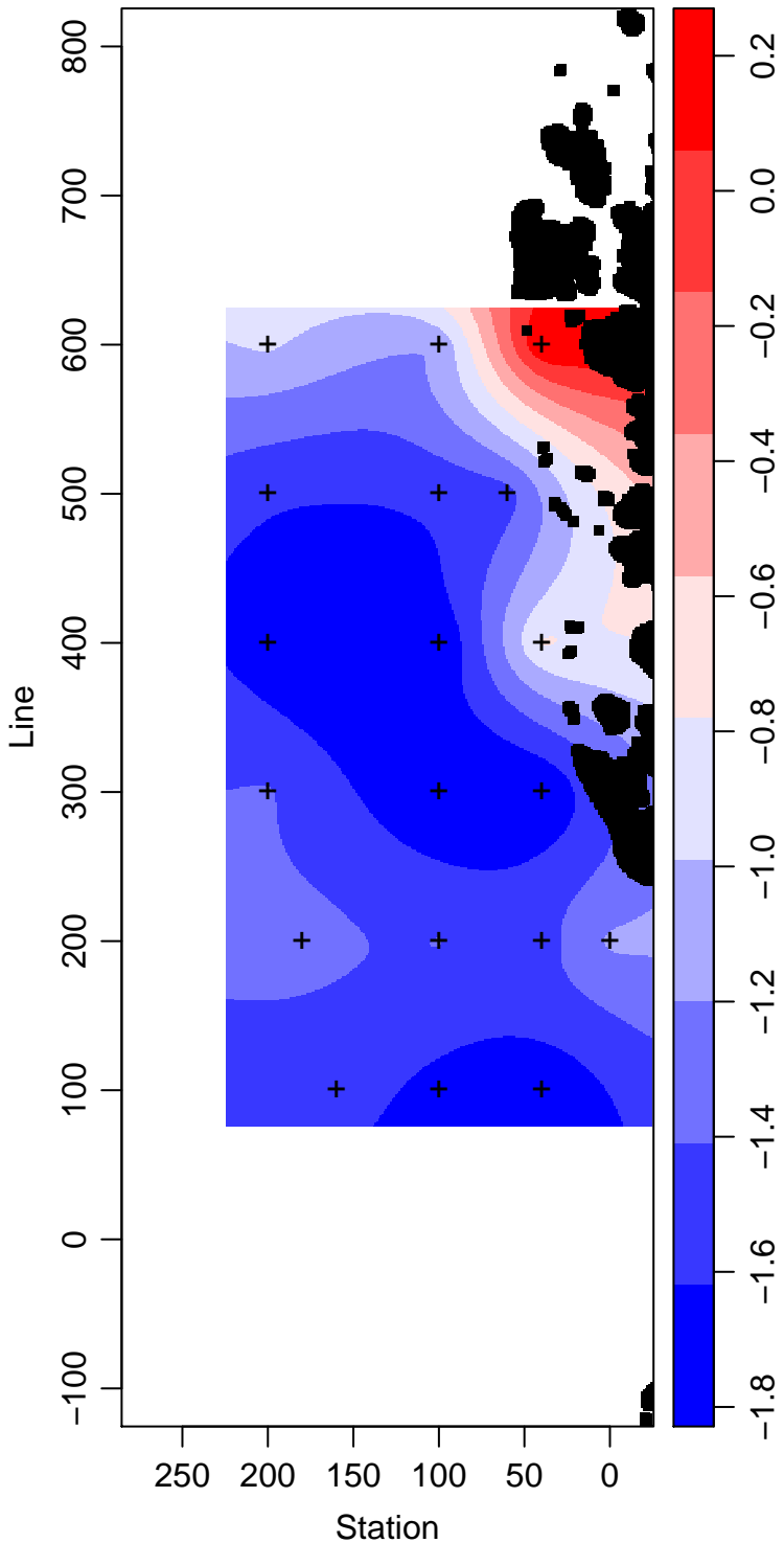
LMG14-01_80_Temperature ° Celsius
