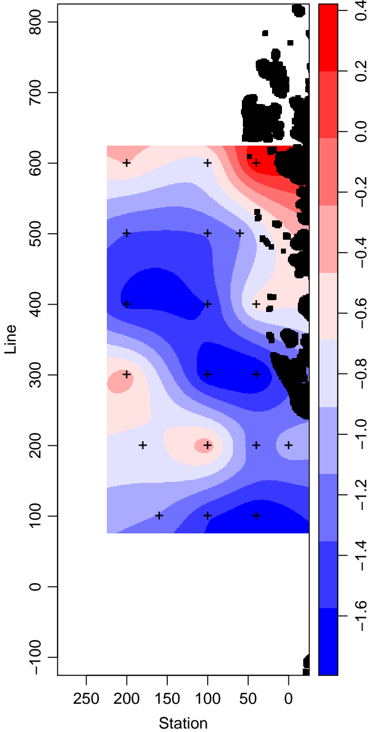
LMG14-01_95_Temperature ° Celsius
