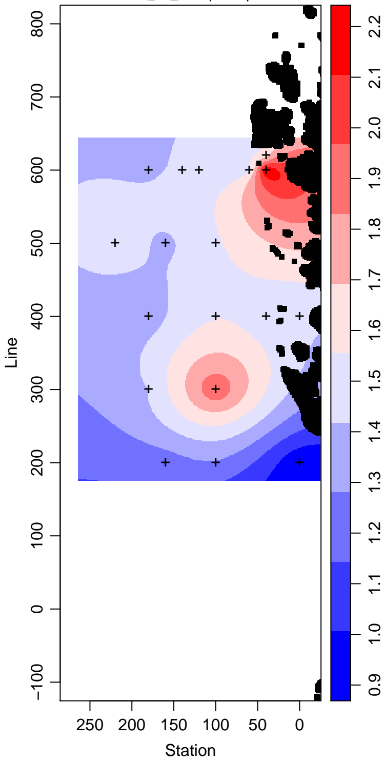
LMG99-01_10_Phosphate \mu\text{ mol L}^{-1}
