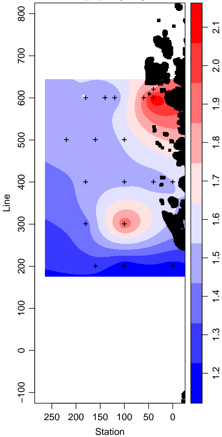
LMG99-01_20_Phosphate \mu\text{ mol L}^{-1}
