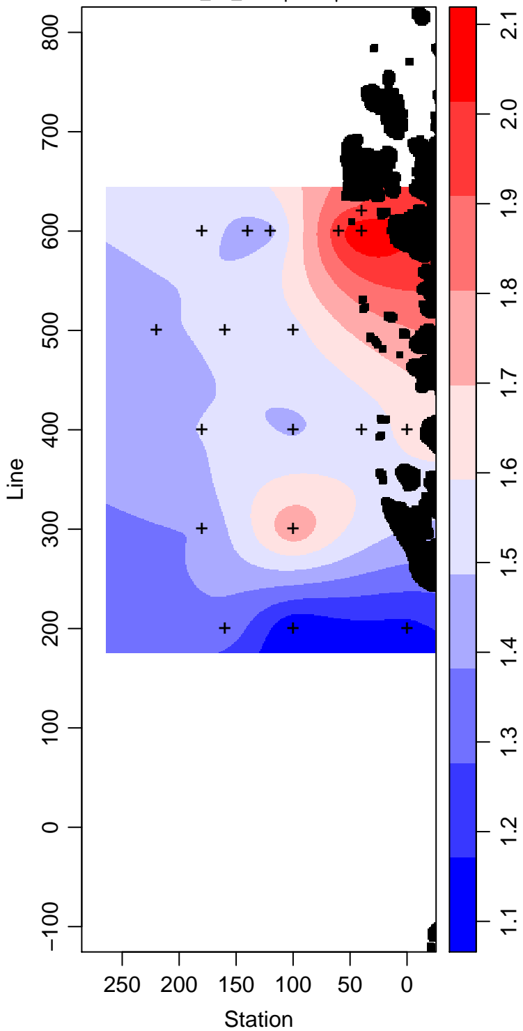
LMG99-01_25_Phosphate \mu\text{ mol L}^{-1}
