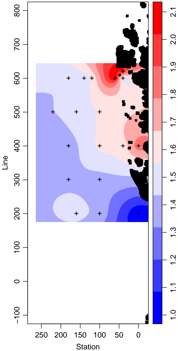
LMG99-01_45_Phosphate \mu\text{ mol L}^{-1}
