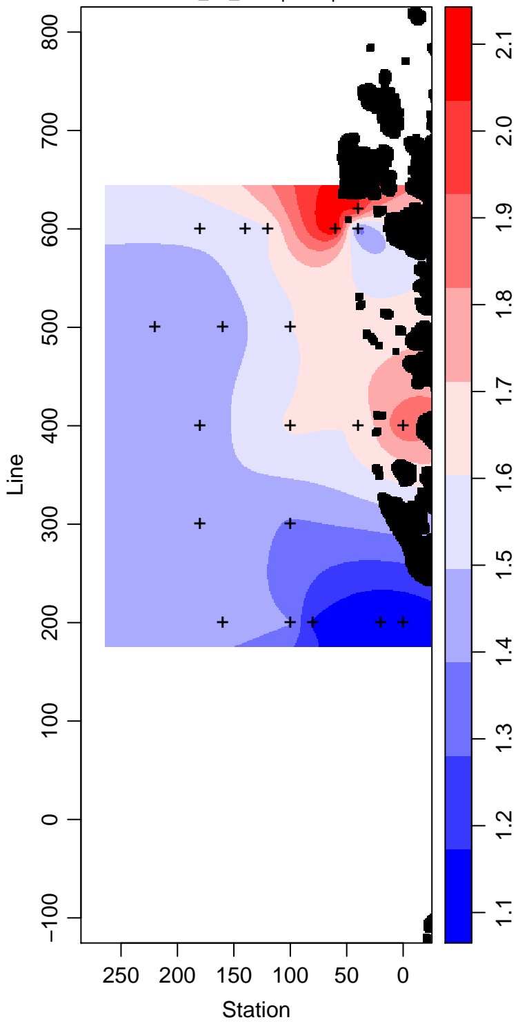
LMG99-01_50_Phosphate \mu\text{ mol L}^{-1}
