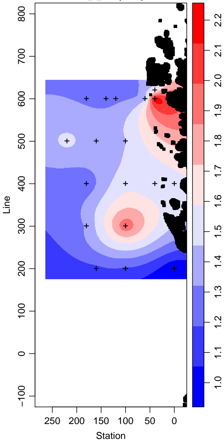
LMG99-01_5_Phosphate \mu\text{ mol L}^{-1}
