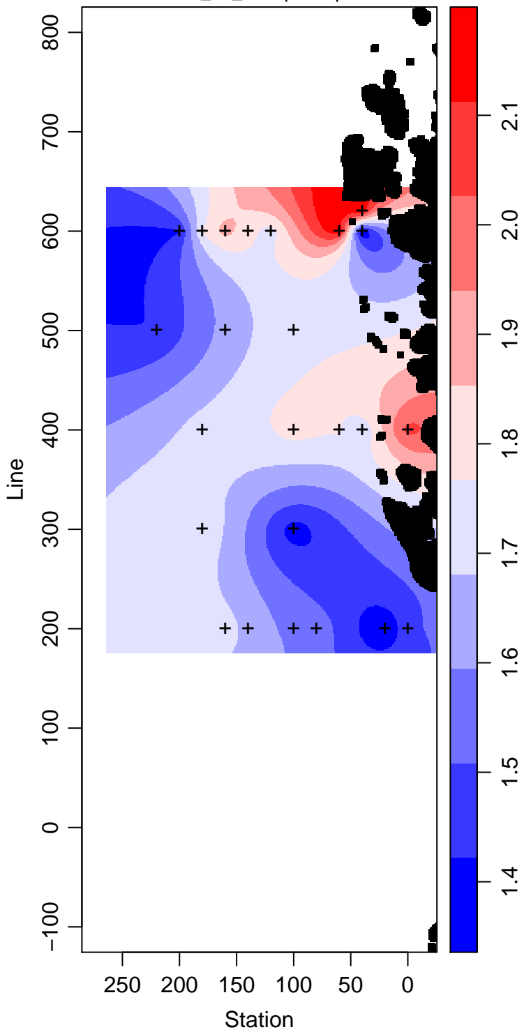
LMG99-01_70_Phosphate \mu\text{ mol L}^{-1}
