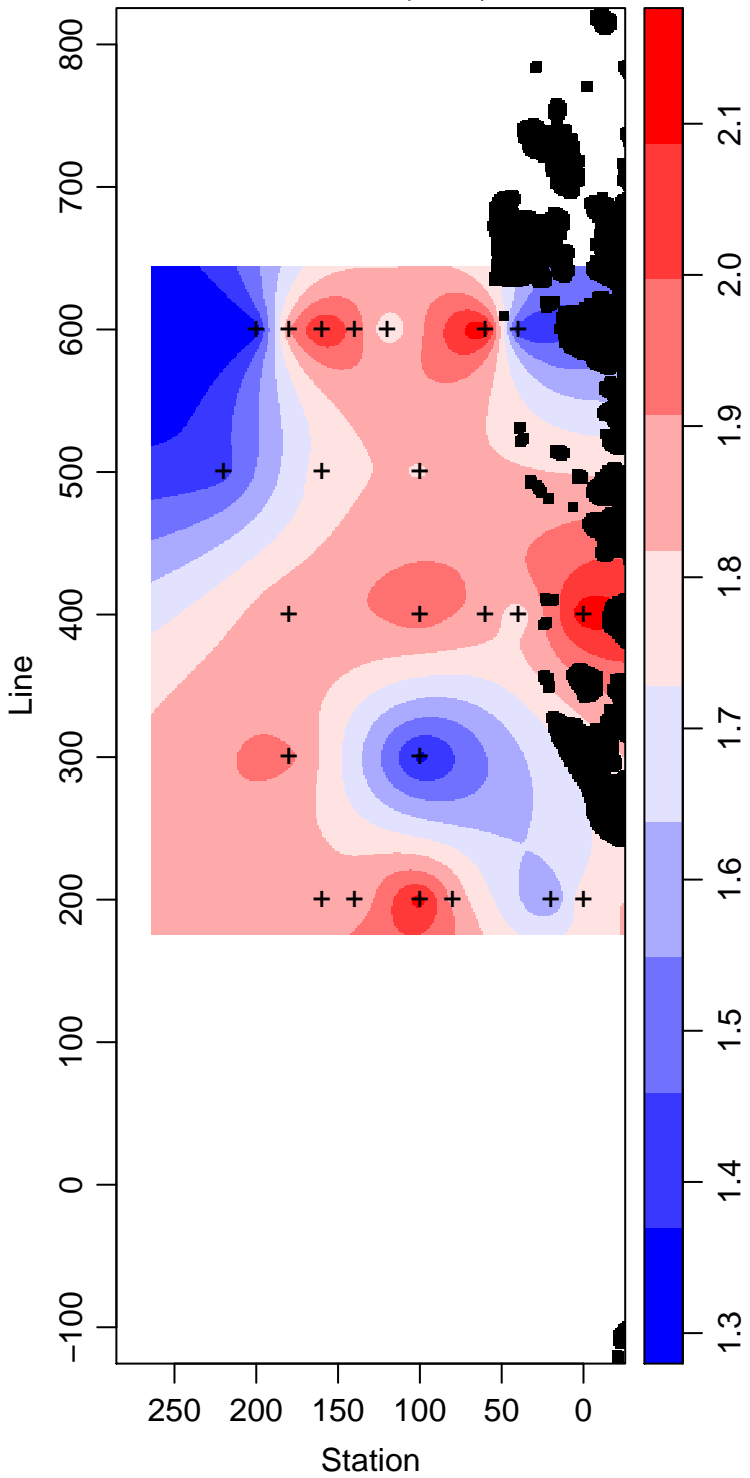
LMG99-01_85_Phosphate \mu\text{ mol L}^{-1}
