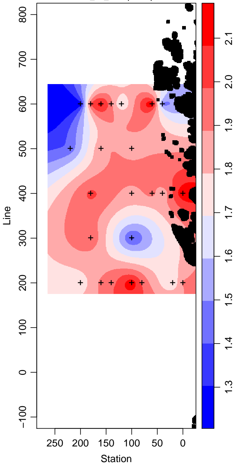
LMG99-01_95_Phosphate \mu\text{ mol L}^{-1}
