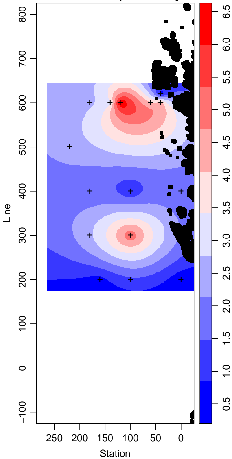
LMG99-01_40_Primary.Production mg m -3
